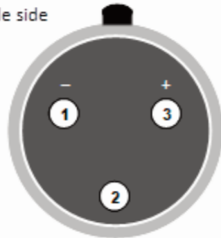
Female – for connection to upper (male) Gemini Mini-XLR socket
