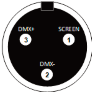
Male – for connection to lower (female) Gemini Mini-XLR socket
